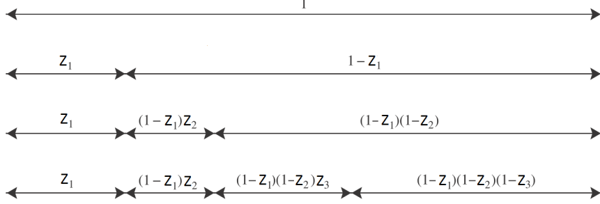
Figure 4: Rescaled stick-breaking: each remaining stick is broken, relatively to its length, by z_i \in [0, 1] .
