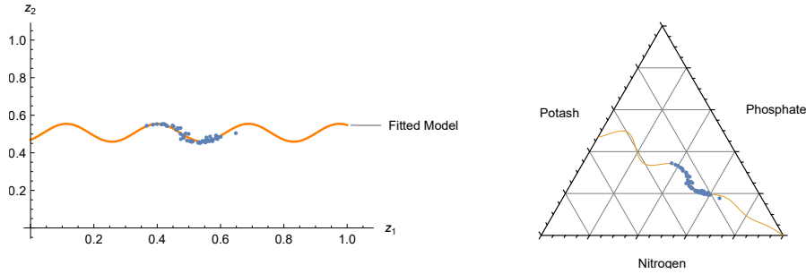
Figure 16: Internal parametric regression model for agriculture data. Scatter plots (blue points) and fitted sinusoidal model (orange line) in the \mathbf{z} space (left) and for the original data (right).
