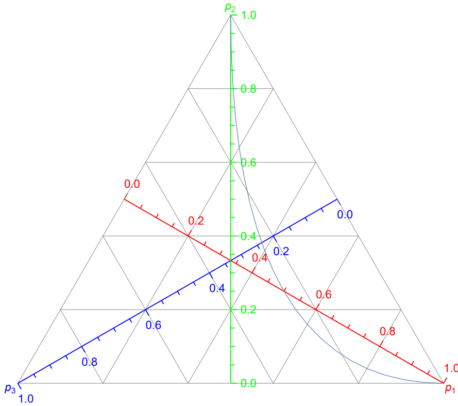
Figure 14: Ternary plot of a CoDa with countermonotone CoDapula and uniform quantile functions, d = 3 , with barycentric axes p_1 (red), p_2 (green), p_3 (blue).
