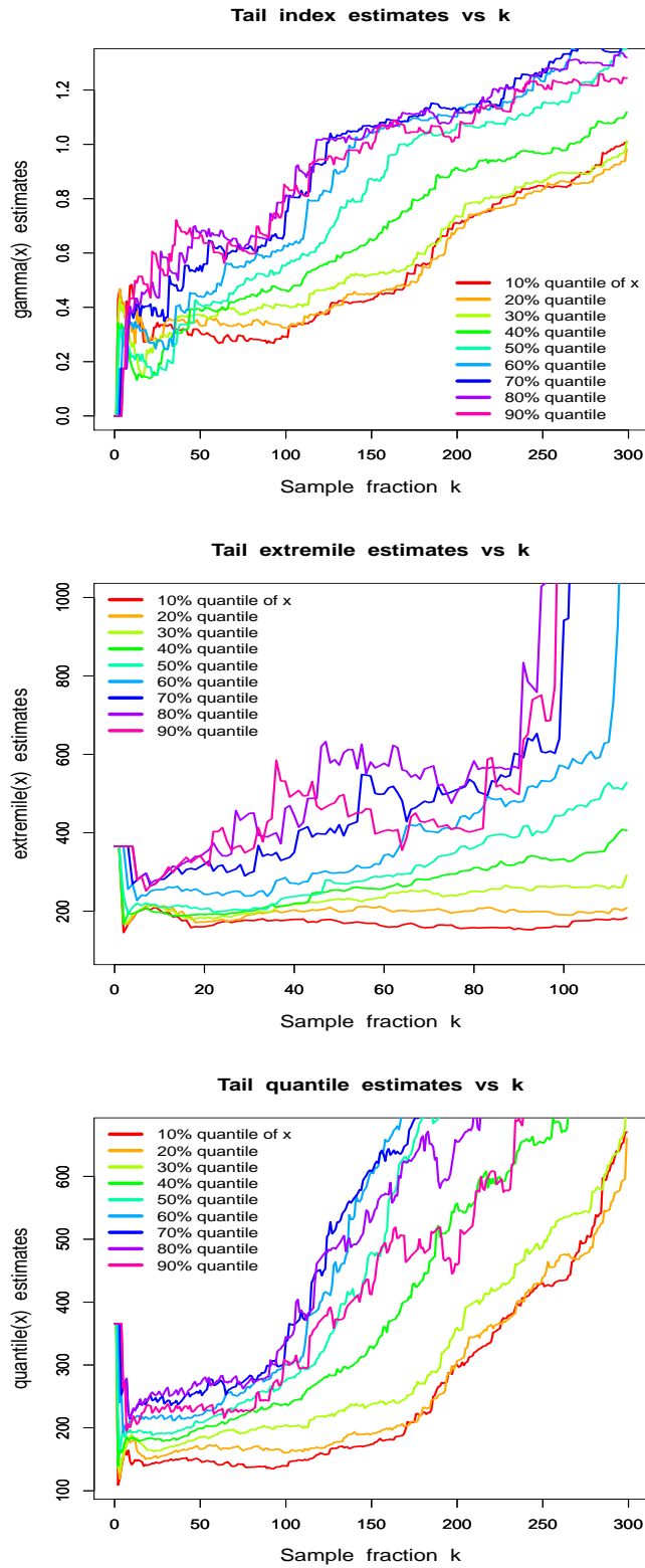
Figure 1: (Top) plots of \hat{\gamma}(x) versus k , (Middle) plots of \hat{\xi}_{.99}(x) versus k , (Bottom) plots of \hat{q}_{.99}(x) versus k , for the 10%, 20%, ..., 90% empirical quantiles x of X .
