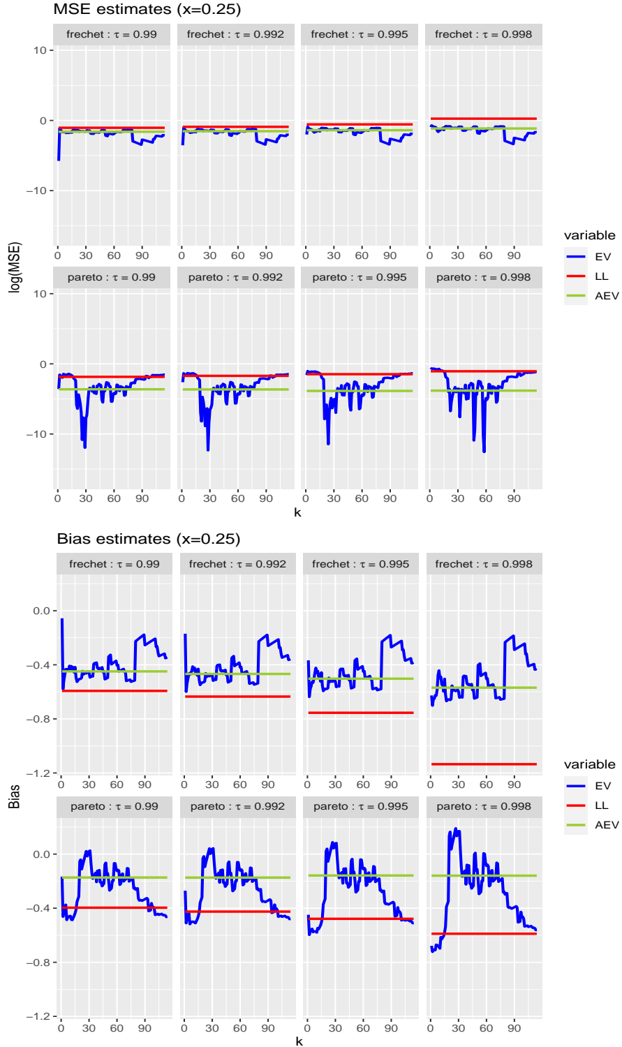
Figure 2: Averaged MSE in log-scale (top) and bias (bottom) of \check{\xi}_{LL, \tau'_n}(x)/\xi_{\tau'_n}(x) in red (LL) and \hat{\xi}_{\tau'_n}^*(x)/\xi_{\tau'_n}(x) in blue (EV) versus k , computed for x = 0.25 over 200 Monte Carlo simulations. In green (AEV), MSE and bias of the average of the Monte Carlo estimates (EV) within the selected stable region.
