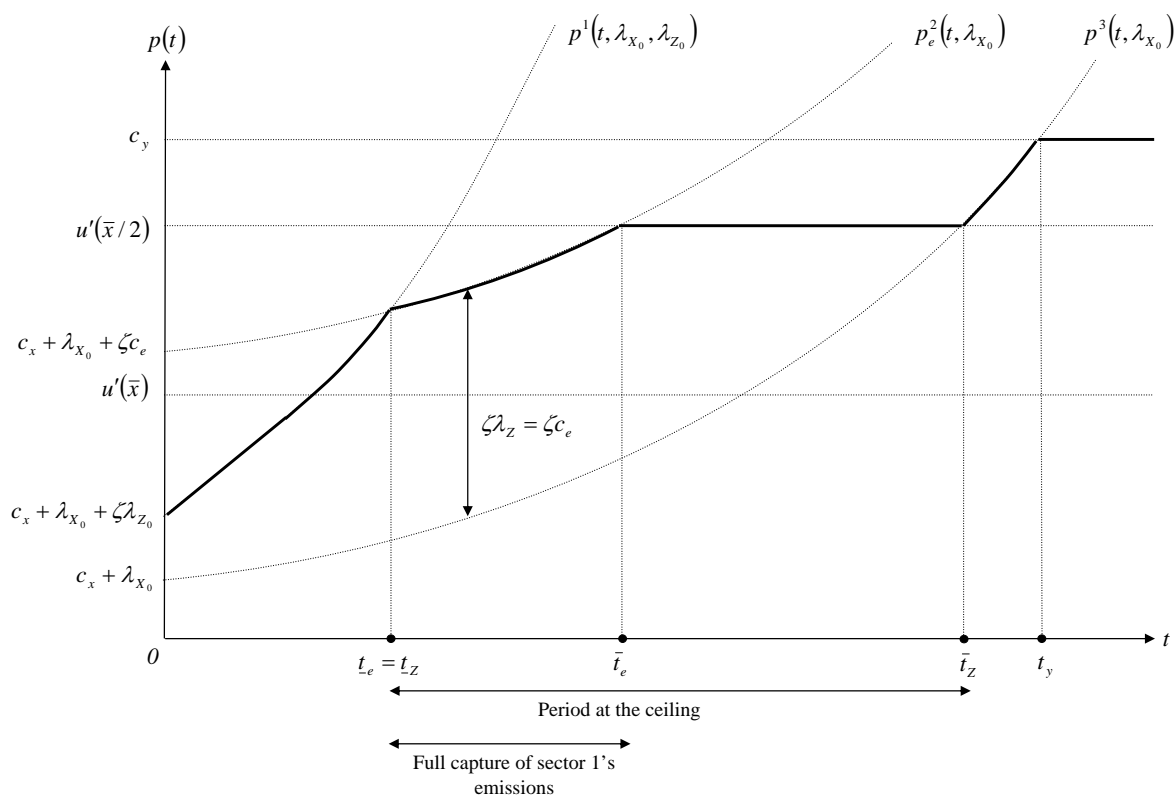
Figure 2: Optimal path along which the energy price is the same for each sector and it is optimal to abate sector 1's emissions
