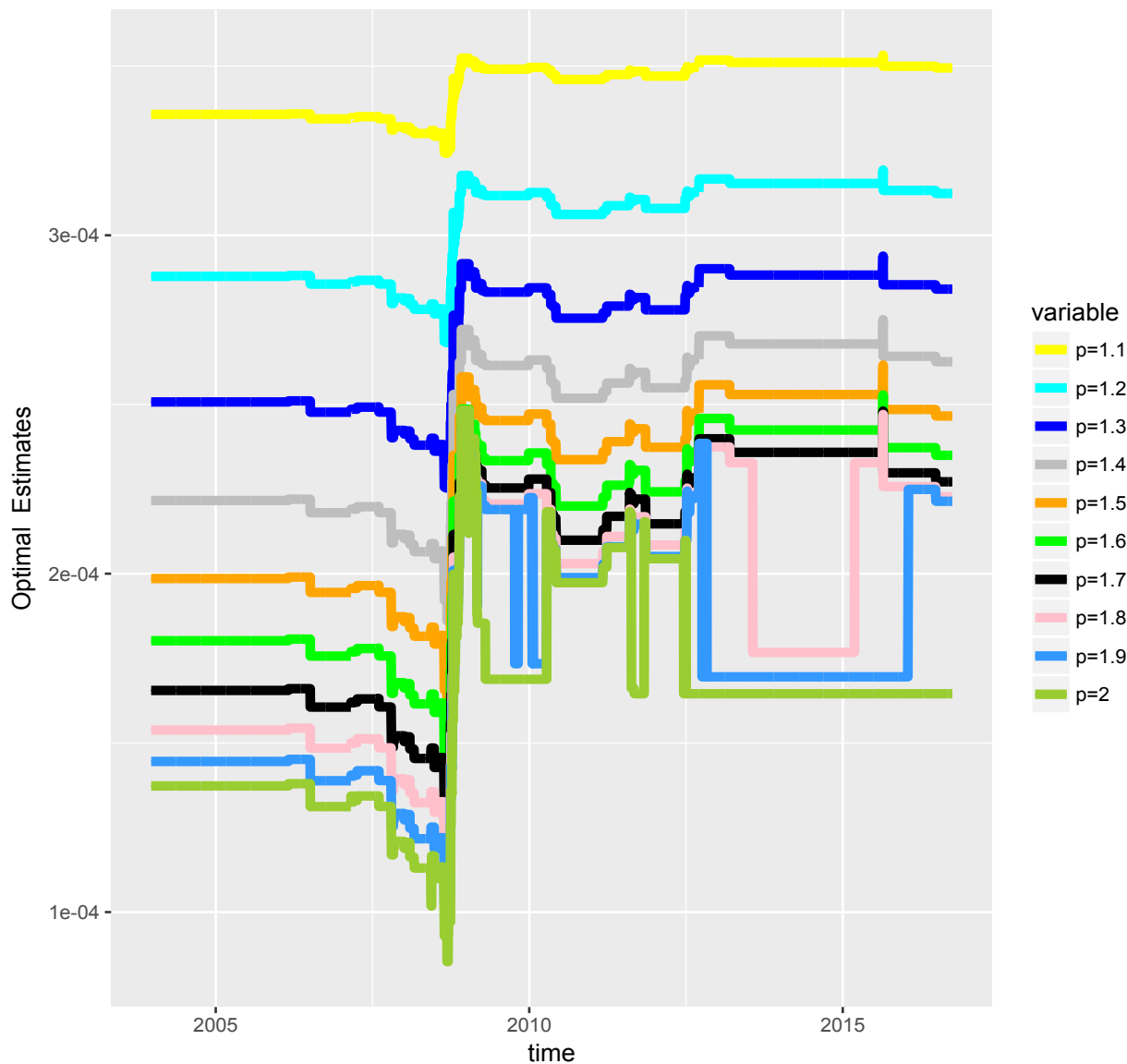
Figure 18: The final estimates t \mapsto \hat{\tau}'_n(t) , obtained for p \in \{1.1, 1.2, \dots, 1.9, 2\} .
