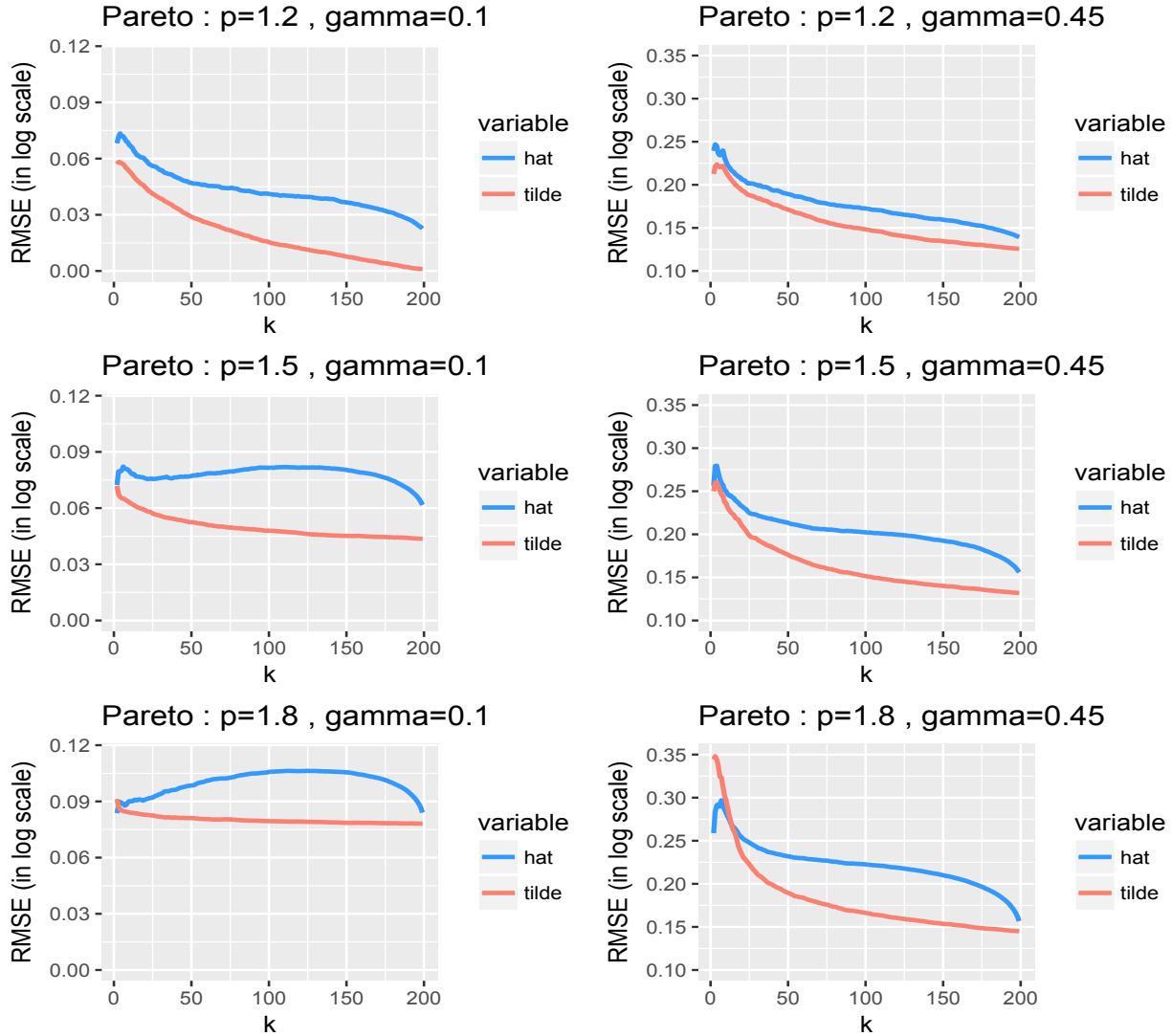
Figure 9: Pareto distribution —RMSE (in log scale) of \hat{q}_{\tau_n}^W(p) (blue) and \tilde{q}_{\tau_n}^W(p) (red) as function of k \in \{2, \dots, n-1\} . From left to right, \gamma = 0.1, 0.45 . From top to bottom, p = 1.2, 1.5, 1.8 .
