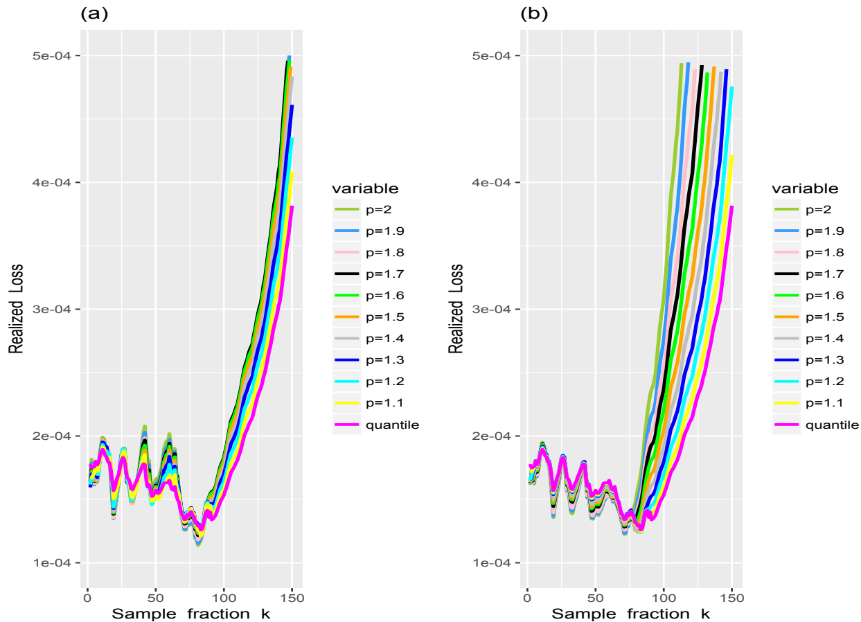
Figure 19: (a)—Plots of the realized loss k \mapsto \bar{L}_n^{(m)}(k) for \hat{q}_{1/n}^W(1) in magenta and \hat{q}_{\tau_n}^W(p) with different values of p . (b)—Results with \tilde{q}_{\tau_n}^W(p) in place of \hat{q}_{\tau_n}^W(p) . Results based on weekly loss returns.
