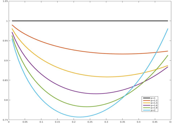
Figure 1: Behavior of \gamma \in (0, 1/2] \mapsto C(\gamma; p) for some values of p \in [1, 2] .
