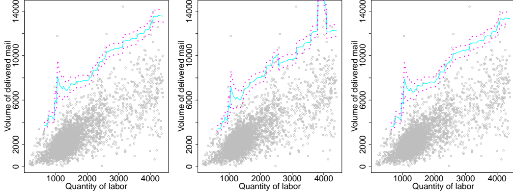
Figure 11: Resulting regularized PWM estimator \tilde{\varphi}_{pwm} and 95% confidence interval of \varphi for the 4000 French post offices. From left to right, we have the case \rho_x = 2 , plugging \bar{\rho}_x and plugging the mean of \bar{\rho}_x .
