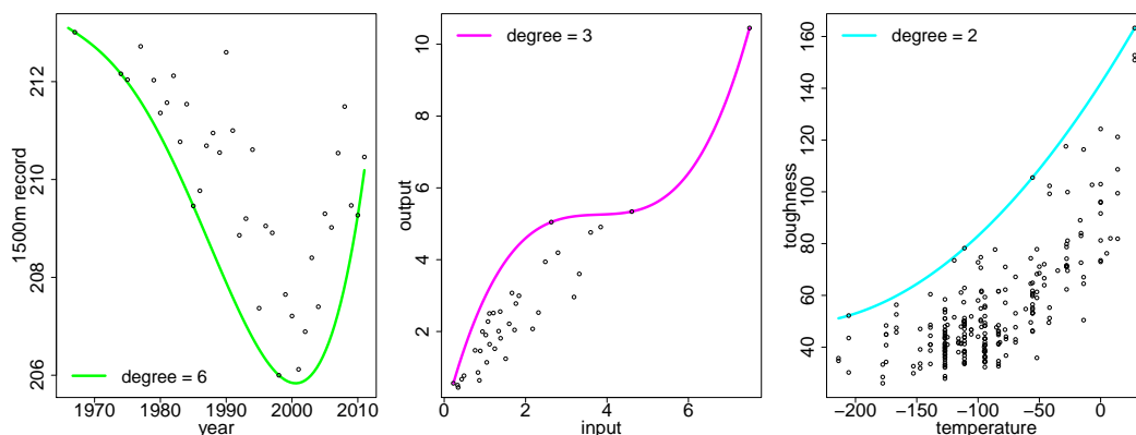
Figure 3: Polynomial boundary estimators for the 46 annual sport records (left), the 37 European air controllers (middle) and the 254 nuclear reactors' data (right).
