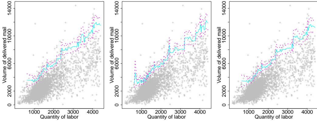
Figure 10: Resulting Pickands estimator \hat{\varphi}_{pick} and 95% confidence interval of \varphi for the 4000 French post offices. From left to right, we have the case \rho_x = 2 , plugging \hat{\rho}_x , and plugging the mean of \hat{\rho}_x .
