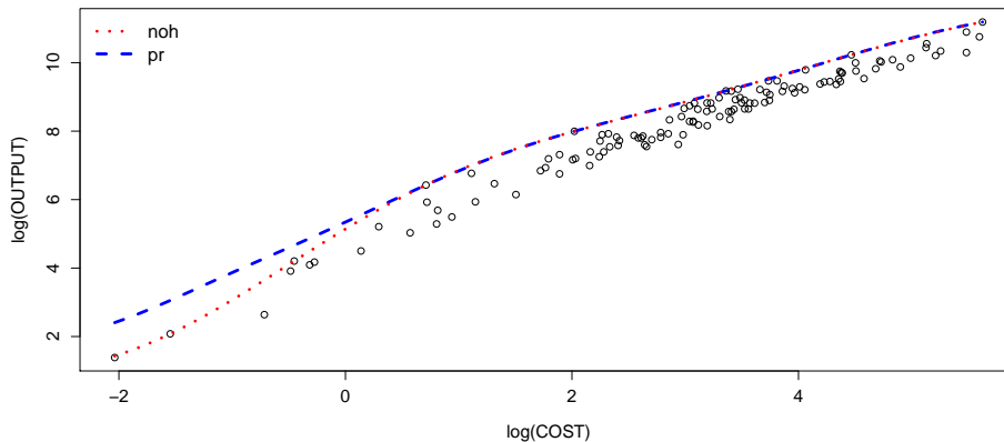
Figure 8: The two kernel smoothing frontier estimators for 123 American electric utility companies.
