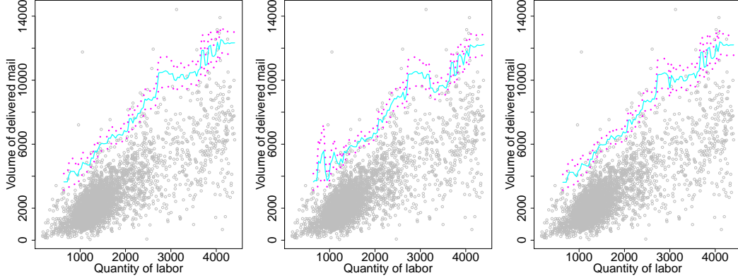
Figure 9: Resulting moment estimator \tilde{\varphi}_{momt} and 95% confidence bands of \varphi for the 4000 French post offices. From left to right, we have the case \rho_x = 2 , plugging \tilde{\rho}_x and plugging the mean of \tilde{\rho}_x .
