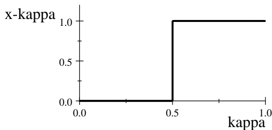
Figure 2: The set of homo-moralis strategies, when (T, R, P, S) = (5, 4, 3, 2) .
