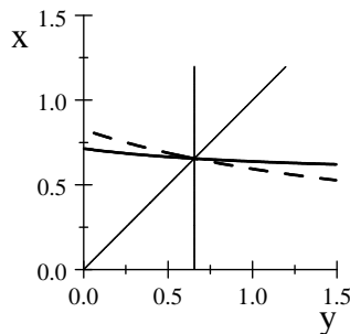
Figure 6: Best-reply curves in a public goods game with b = 0.5 and c = 1 , for a homo moralis with \kappa = 0.5 (solid) and an altruist with \alpha = 0.5 (dashed).
