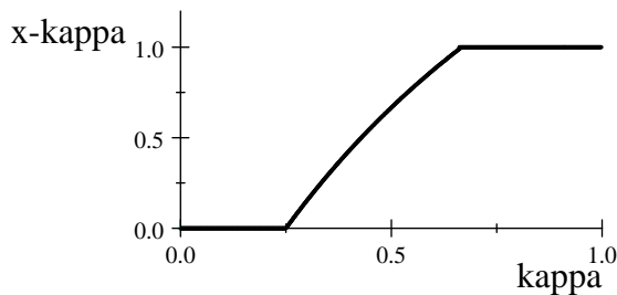
Figure 3: The (singleton) set of homo-moralis strategies for (T, R, P, S) = (7, 5, 3, 2) .
