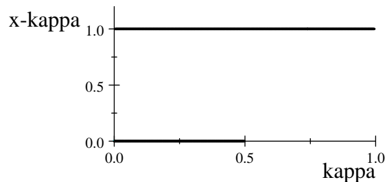
Figure 5: The set of homo-moralis strategies, for a = 2b .
