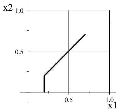
Figure 1: The set of Hamiltonian strategies in the ultimatum-bargaining fitness game.
