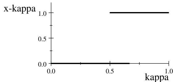
Figure 4: The set of homo-moralis strategies, for (T, R, P, S) = (5, 4, 3, 1) .
