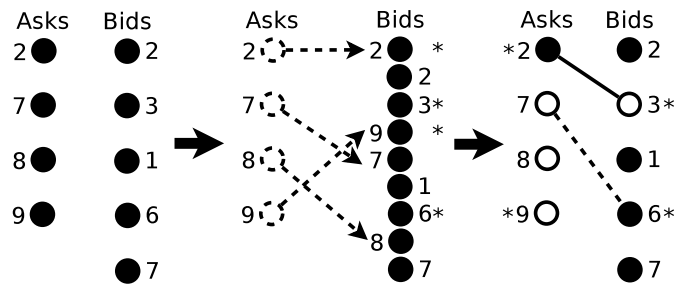
FIGURE 6.7: A Running Example of \mathcal{M}_{\mathcal{A}}
