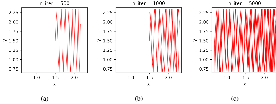
Figure 6: Gradient path after (a) 500, (b) 1000 and (c) 5000 iterations.
