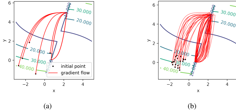
Figure 5: (a) Gradient flows for several initializations. (b) Gradient flows for 20 perturbed experiments with \sigma^2 = 0.4 .
