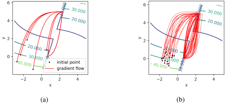
Figure 2: (a) Gradient flows for several initializations. (b) Gradient flows for 20 perturbed experiments with \sigma^2 = 0.4 .
