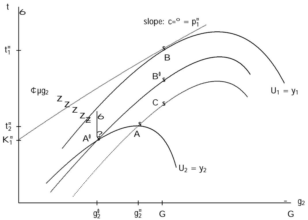
Figure 1: Full information optimum (A; B) and optimum under asymmetric information ( A^0 ; B^0 ). Both solutions are for regime i) and the financial constraints are ignored.
