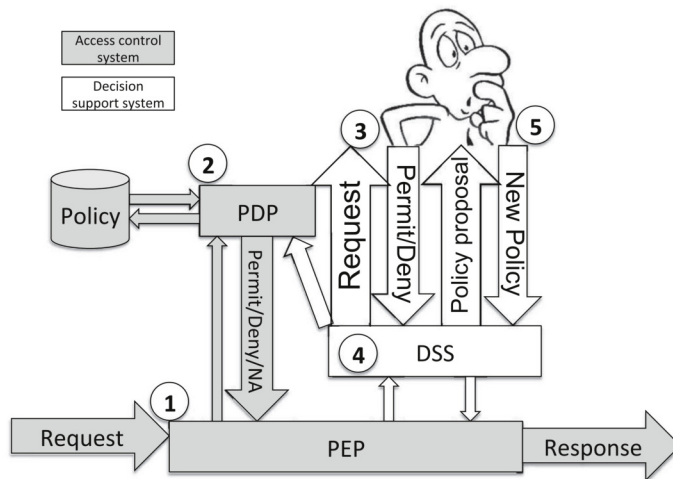
Fig. 4 KAPUER's architecture integrated in XACML
