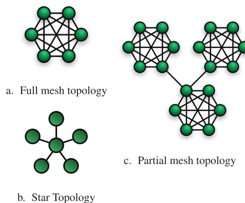
Figure 1: Peer-to-peer topologies
